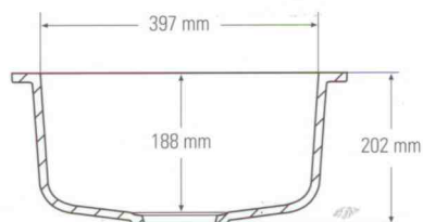
Side cross-section
